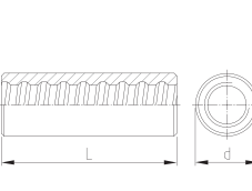
Muffe standard coupler standard
