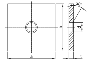
Ankerplatte Konus 30° groß anchor plate cone 30° big
